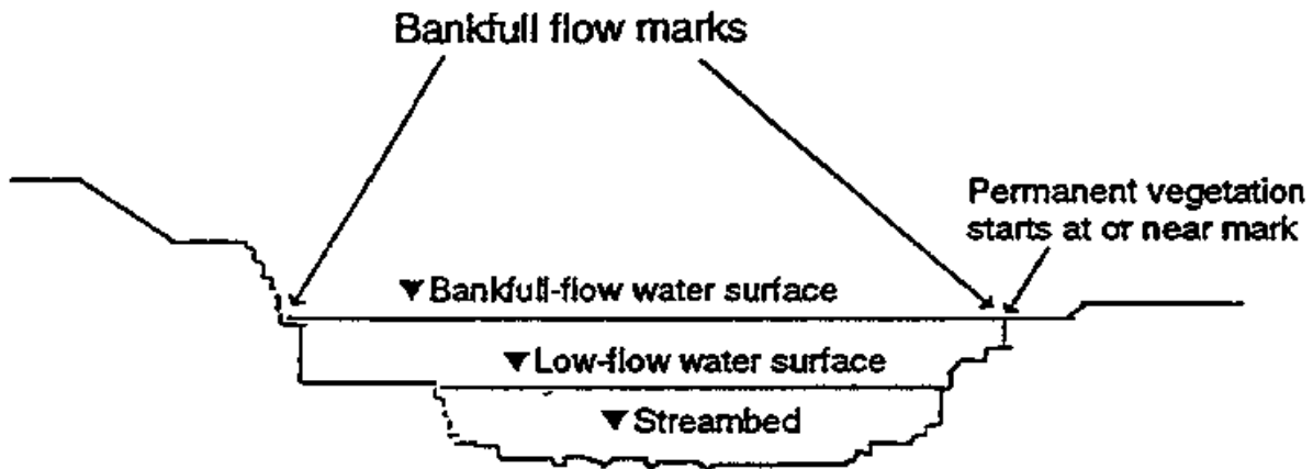
Figure 2. Location of bankfull width marks.
